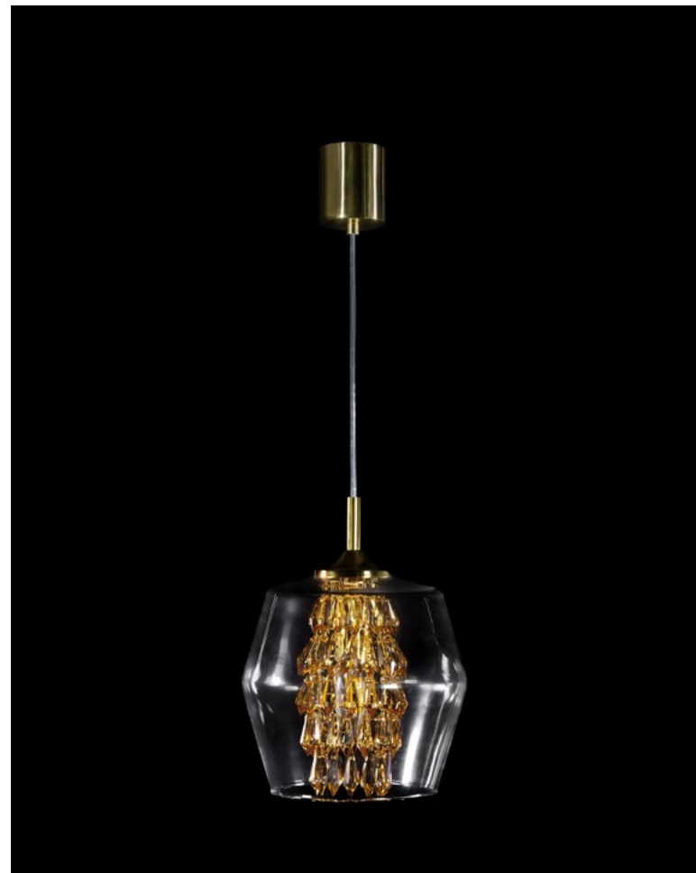
FORM 01-CH-PB-CL DROPS - 8003 | Ø 200 x H 200 (TH 1500) mm | 1 x E14
